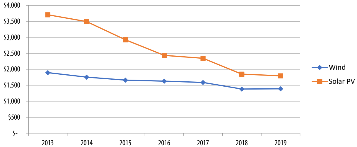
Figure 4. U.S. capacity-weighted average construction costs, $/kW
