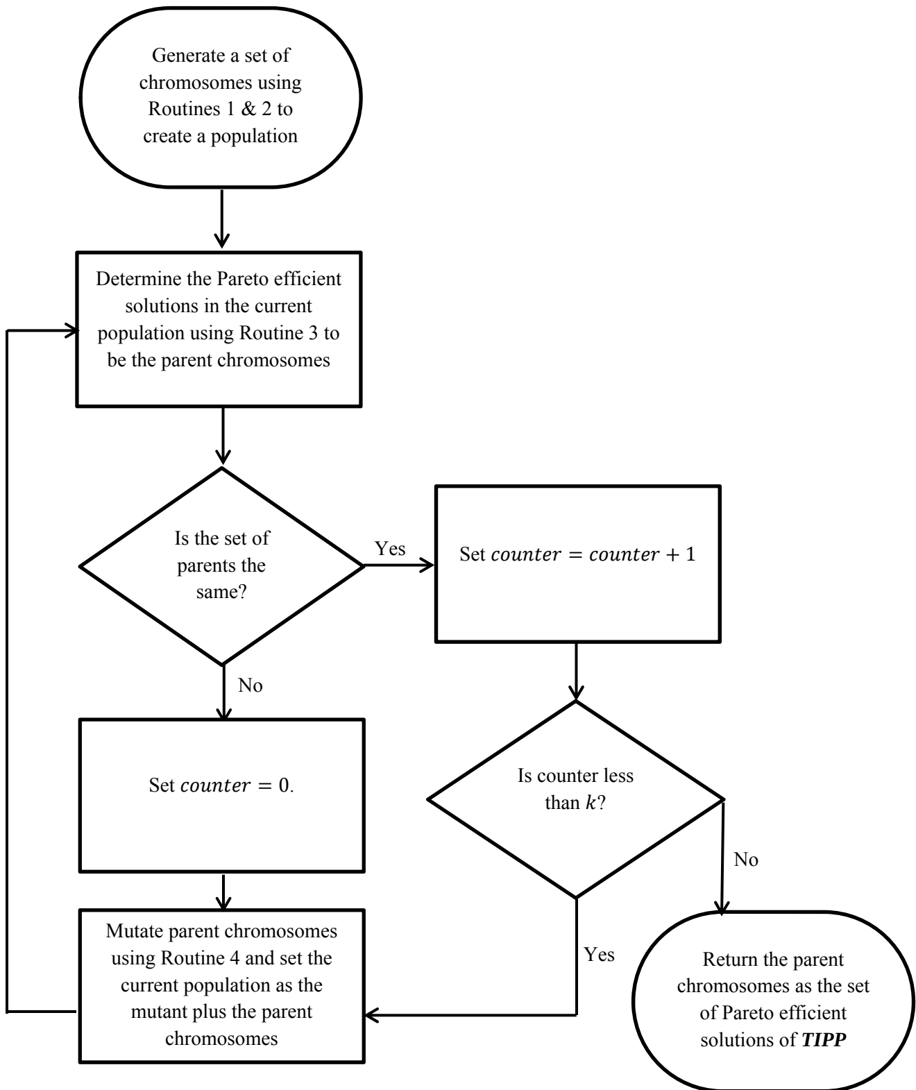
Figure 3. Genetic Algorithm Flow Chart
