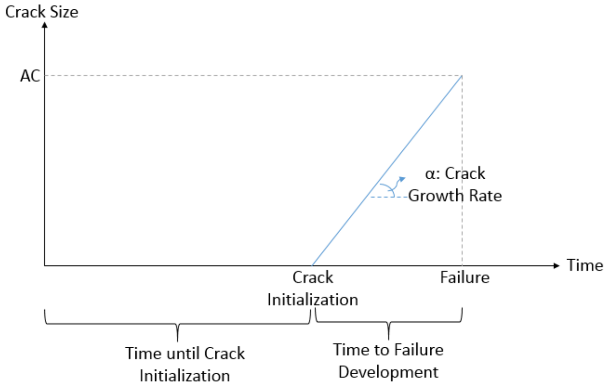
Figure 13. Crack Growth over Time
