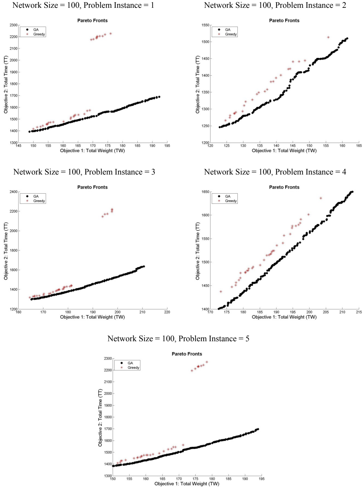
Figure 7: Pareto Fronts of the Genetic and Greedy Algorithms
