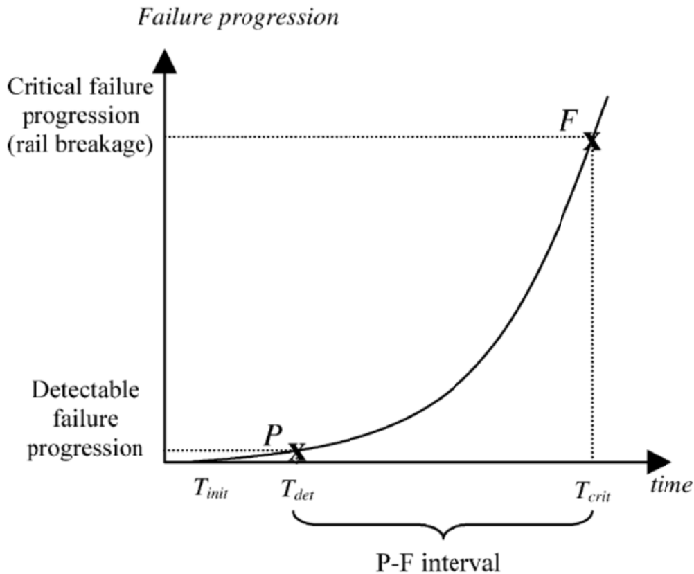
Figure 10. P-F Interval Illustration (Podofillini et al., 2006)
