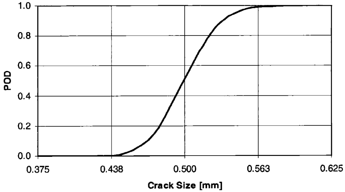
Figure 12. Lognormal Detection Probabilities of Cracks (Kashima, 2004)
