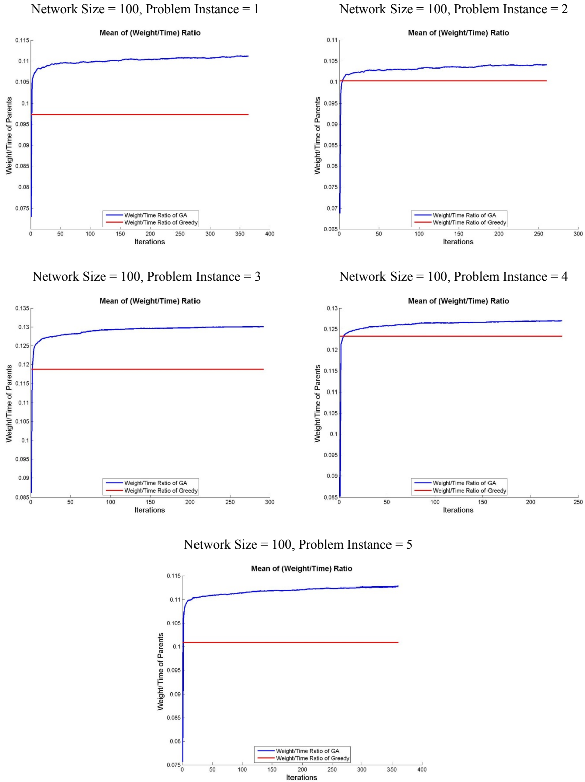
Figure 6: Average TW/TT Ratios vs. Iterations
