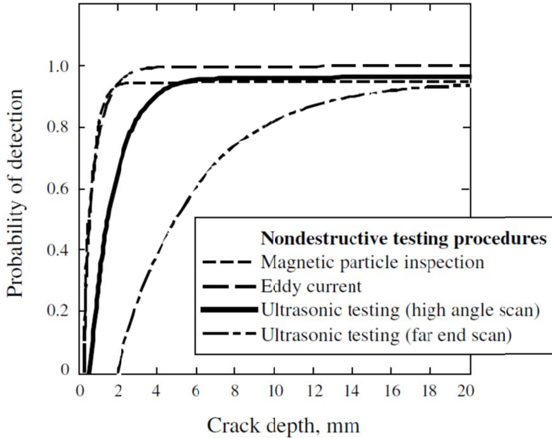
Figure 11. Detection Probabilities for Different Inspection Methods (Zerbski et al., 2005)
