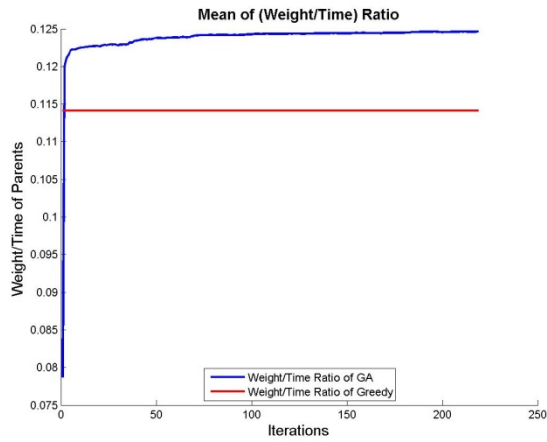
Network Size = 300, Problem Instance = 3
