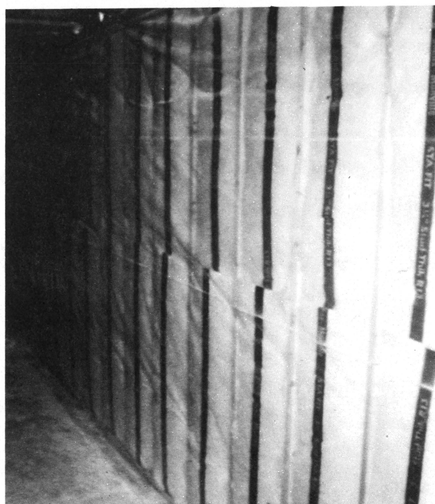
Figure 3. This well insulated exterior wall section contains 3½-inch-thick fiber glass batts. A clear polyethylene sheet has been placed over the batts to act as a vapor barrier. Clear polyethylene provides an excellent vapor barrier and has good transparency so carpenters or dry wall installers can see stud faces easily when they apply the interior wall covering. A one-inch thick expanded polystyrene sheathing board on the outside surface of the studs brings total R-value for wall insulation to 18.
