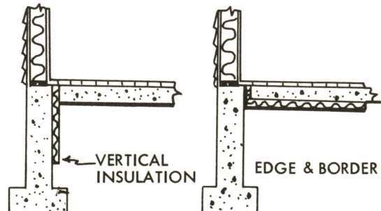
Figure 1. Two different ways of installing rigid foam plastic insulation at the edge of exposed concrete slabs.
