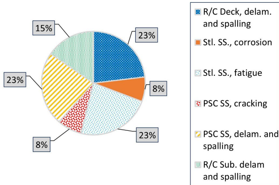
Figure 2.13. Distribution of controlling damage modes for CR \geq 7 bridges without considering the impact damage mode.
