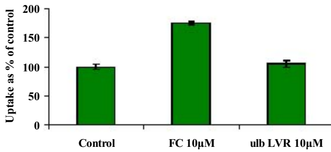
Figure 3: Intracellular accumulation of [3H] MX in MDCKII-Bcrp1 cells
