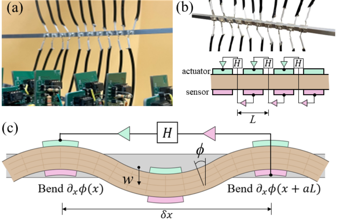
Figure 4.1: Design and mechanics of a nonlocal micropolar metabeam. (a) A photograph of the proposed nonlocal micropolar metabeam with a programmable electronic microcontroller system in the foreground. The host beam is 5 mm wide and 3 mm thick. It is made of aluminum ( \rho_b=2700 kg/m 3 , G_b=26 GPa, E_b = 69 GPa). All the piezoelectric patches mounted on the beam are PZT-AJ ( \rho_p=7600 kg/m 3 , \epsilon_{33}^T = 1900\epsilon_0 , d_{31} = -1.75 \times 10^{-10} C/N, d_{33} = 4 \times 10^{-10} C/N, d_{15} = 5.9 \times 10^{-10} C/N) with a thickness of 0.64 mm, a side length of 6.4 mm and a width of 4.9 mm. (b) An illustration of the full nonlocal metabeam, later used in the experiments, is shown in the top panel. The bottom panel shows the schematic of a segment of the metabeam. The top and bottom piezoelectric patches serve as actuators and sensors, respectively. They are connected beyond nonlocally by the transfer function H . The illustrated example here corresponds to a nearest-neighbor nonlocal configuration. The lattice constant is L = 10 mm. (c) Schematic illustration of the mechanics of the nonlocal micropolar metabeam. The motion of the metabeam can be described by two independent micropolar degrees of freedom: flexural displacement w and rotation angle \phi . The (n + a) th sensor is connected to the n th actuator through H in a periodic way. This equivalently means the nonlocal bending at x + \delta x , where \delta x = aL , is modulated by H and then contributes to the local bending at x .
