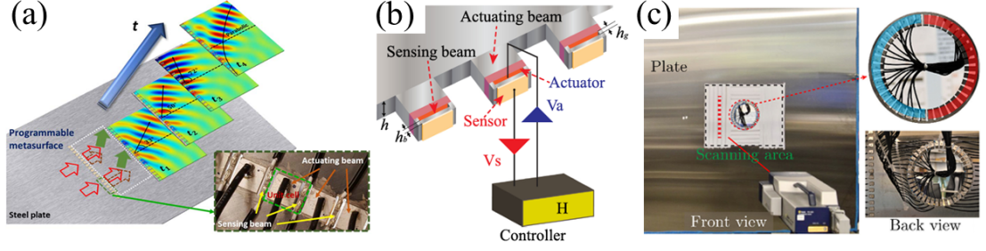
Figure 1.4: Active elastic metasurfaces enabled by reprogrammable piezoelectric shunts. (a) A reprogrammable metasurface capable of conducting real-time control of broadband elastic rays [50]. (b) A piezoelectric-based programmable meta-boundary that shapes elastic wave mode conversion [51]. (c) Optimal flexural wave absorption and cloaking with an active meta-layer [52].
