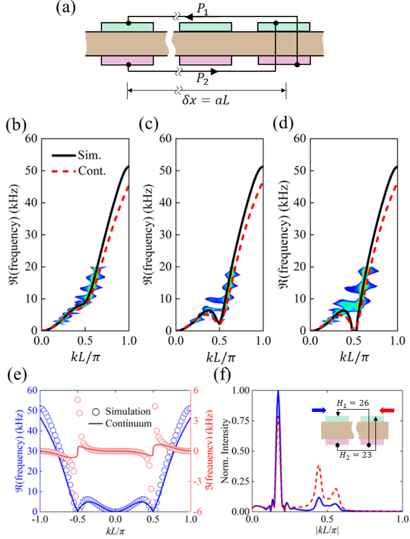
Figure 4.6: Reciprocal and nonreciprocal roton-like dispersions. (a) Schematic illustration of the nonlocal realization of the roton-like dispersion with a toggle between reciprocity and nonreciprocity. (b-d) Reciprocal roton-like dispersion relations enabled by H_1 = H_2 = H or equivalently P_1 = P_2 = P . The change of the \Re(\omega) band is shown when H = 20 , H = 23.5 , and H = 24 , or numerically P = 3.08 \times 10^4 \text{ kgm}^2/\text{s}^2 , P = 4.09 \times 10^4 \text{ kgm}^2/\text{s}^2 and P = 4.2 \times 10^4 \text{ kgm}^2/\text{s}^2 under the continuum limit. The black and red curves represent the eigenfrequency simulation and continuum theory. The color fills are the FFT results. (e) Nonreciprocal roton-like dispersion relations enabled by H_1 = 26 and H_2 = 23 or equivalently P_1 = 4.34 \times 10^4 \text{ kgm}^2/\text{s}^2 and P_2 = 3.95 \times 10^4 \text{ kgm}^2/\text{s}^2 under the continuum limit. Comparison of the complex spectra between simulation and continuum theory is shown. (f) The normalized FFT-based intensity spectrum for the propagation of two opposite directions within the nonreciprocal roton-like configuration are shown at 2 kHz where the nonreciprocal roton-like behavior takes place.
