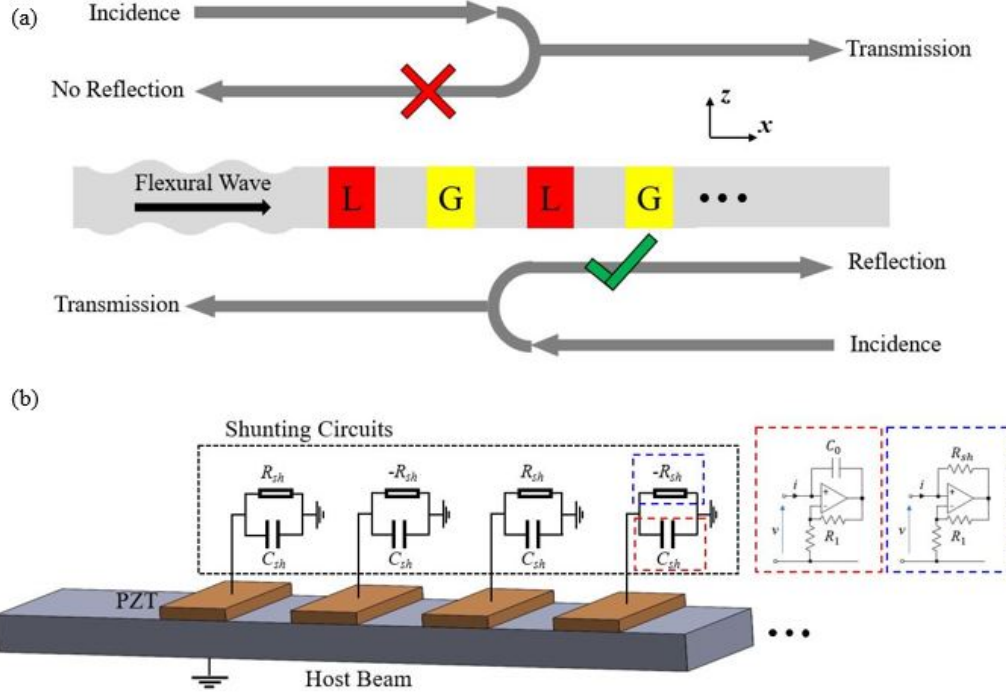
Figure 2.1: (a) Schematic of the non-Hermitian \mathcal{PT} symmetric beam for asymmetric flexural wave scattering. Unidirectional reflectionlessness is illustrated in the figure. (b) Physical realization of the \mathcal{PT} symmetric beam with piezoelectric patches shunted with negative and positive resistances together with a negative capacitance connected in parallel. The insets highlighted in red and blue illustrate the physical realization of the electrical shunting components. Reproduced from The Journal of the Acoustical Society of America 146, 850 (2019), with the permission of AIP Publishing.
