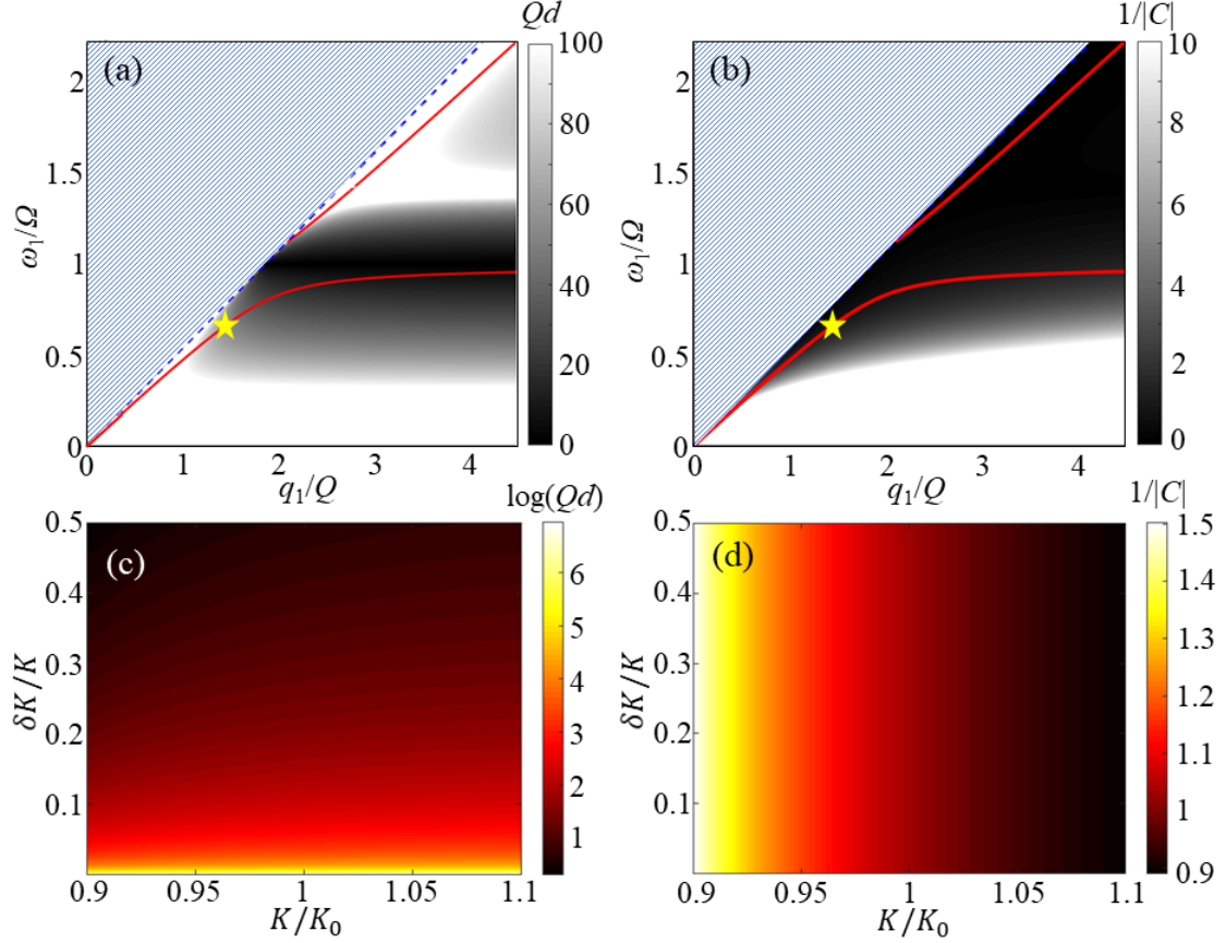
Figure 3.5: Dependence of the normalized conversion length Qd (a) and the inverted amplification factor 1/|C| (b) on (\omega_1, q_1) for an incidence at the mode (\omega_0, q_0) , marked with yellow pentagrams. The pattern-hatched areas denote the bulk regions, and the red curves are the dispersion curves of the Rayleigh wave in the unmodulated system. (c) and (d) show dependence of \log(Qd) and 1/|C| , respectively, on the variations of K and \delta K . Here, K_0 = 2.4 \times 10^3 N/m . Reproduced from Journal of the Mechanics and Physics of Solids 146, 104196 (2021), with the permission of Elsevier Publishing.
