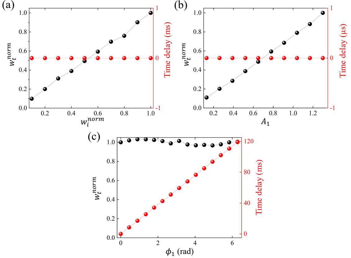
Figure 6.2: Linear independent control over frequency conversion from 10 to 8.5 kHz. Transmitted displacement ratio of wave packets w_t^{norm} and time delay are numerically demonstrated by sweeping (a) maximum incident displacement w_i^{norm} from 0.1 to 1, (b) amplitude A_1 given in Eq. (6.7) from 0.13 to 1.3, and (c) phase shift \phi_1 from 0 to 2\pi . In each cases, the parameters that are not swept remain unchanged as used in Fig. 6.4. Reprinted figure with permission from Q. Wu, X. D. Zhang, P. Shivashankar, Y. Y. Chen, and G. L. Huang, Physical Review Letters , 128, 244301 (2022). Copyright (2022) by the American Physical Society.
