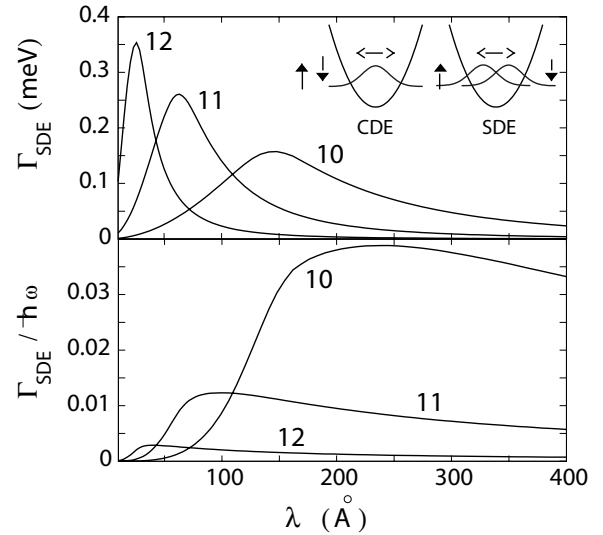
FIG. 2. Upper panel: Spin-plasmon linewidth \Gamma_{\text{SDE}}^{\text{SCD}} for a parabolic quantum well versus curvature parameter \lambda , for N_s = 10^{10} , 10^{11} , and 10^{12} \text{cm}^{-2} and GaAs parameters. The inset illustrates the collective motion of the two spin populations (CDE, in phase; SDE, out of phase). Lower panel: Rescaled linewidth \Gamma_{\text{SDE}}^{\text{SCD}}/\hbar\omega .
