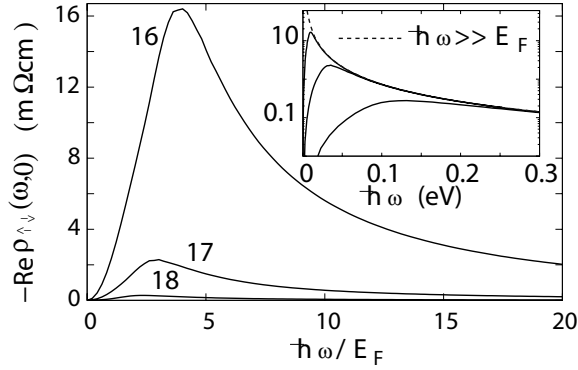
FIG. 1. Spin transresistivity |\text{Re } \rho_{\uparrow\downarrow}| vs rescaled frequency \hbar\omega/E_F for n=10^x \text{ cm}^{-3} , x=16, 17, 18 as indicated and GaAs parameters ( m=0.067m_e , \epsilon=12 ). Inset: |\text{Re } \rho_{\uparrow\downarrow}| in \text{m}\Omega \text{ cm} vs \hbar\omega in \text{eV} for the same densities. Dashed line: high-frequency limit Eq. (6).
