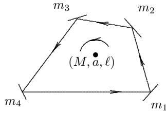
Figure 1. Propagation of null rays along a closed contour around a mass M with gravitomagnetic monopole ( \mu = -\ell ) and dipole ( J = Ma ) moments. The ‘mirrors’ m_1 – m_4 in this schematic diagram could be transponders on-board artificial satellites.
