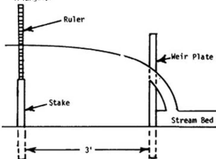
Figure 5 Measuring head on the weir.
