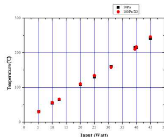
Electrode temperatures during calibration with resistance heater. Black squares, vacuum at 10 Pa; red circles, D 2 gas at 100 Pa.
