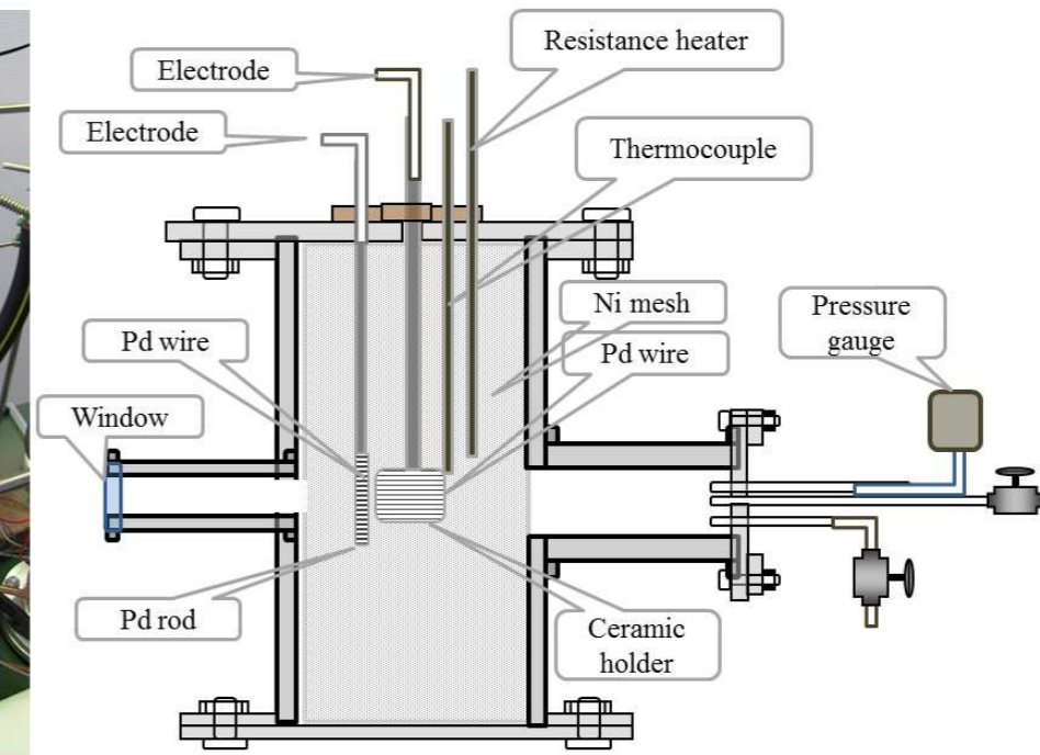
Schematic of reactor
