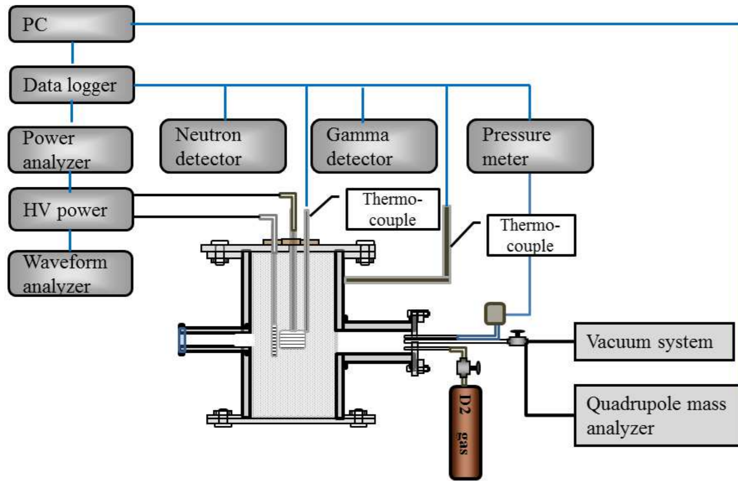
Schematic of equipment setup
