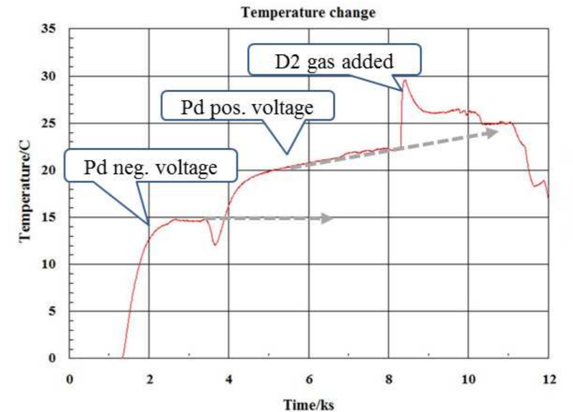
A typical run with a fine wire palladium electrode
