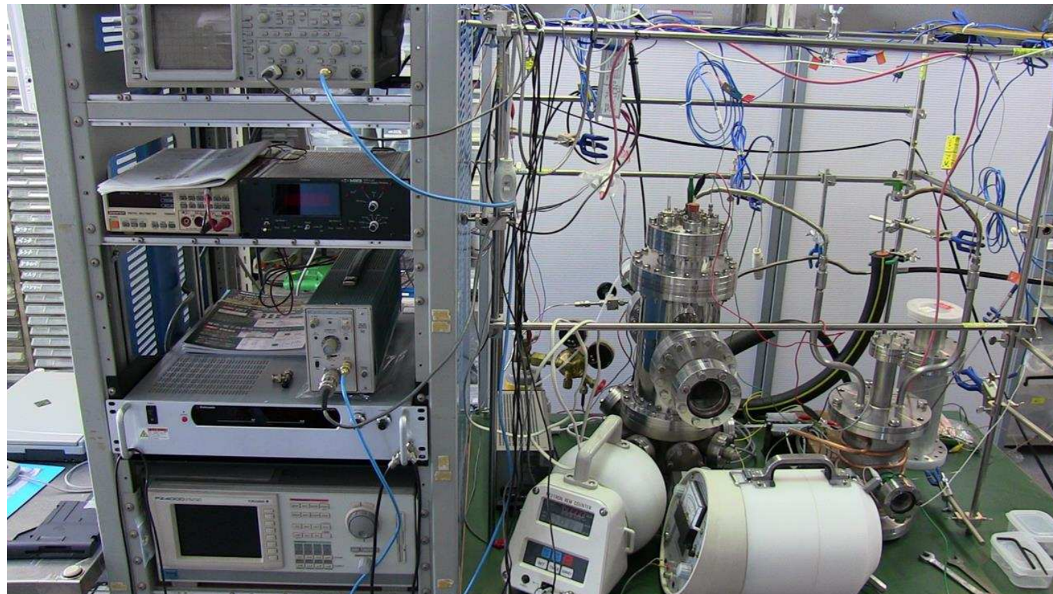
Equipment setup. Radiation detectors are in the foreground.
