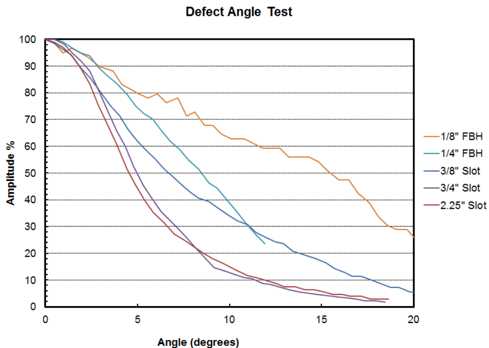
Figure 4-15: Normalized B-Scans relative to transducer rotation
