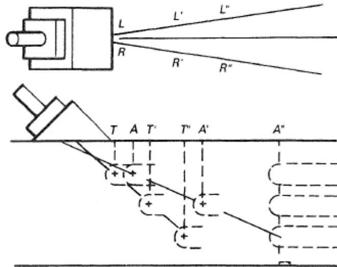
Figure 2-5: Beam spread calibration of the ASME Ultrasonic Code
