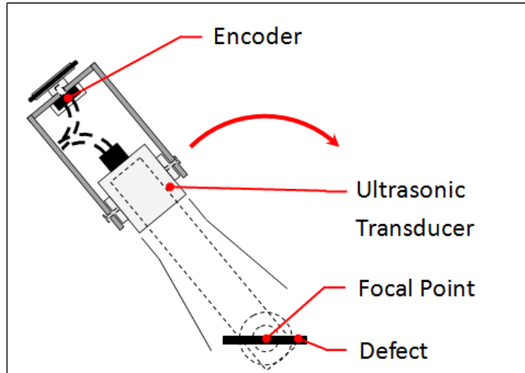
Figure B-3: Defect Angle test setup diagram
