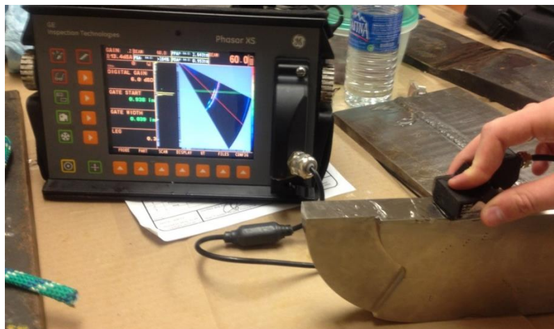
Figure 4-21: PAUT inspection of the phased array IIW block
