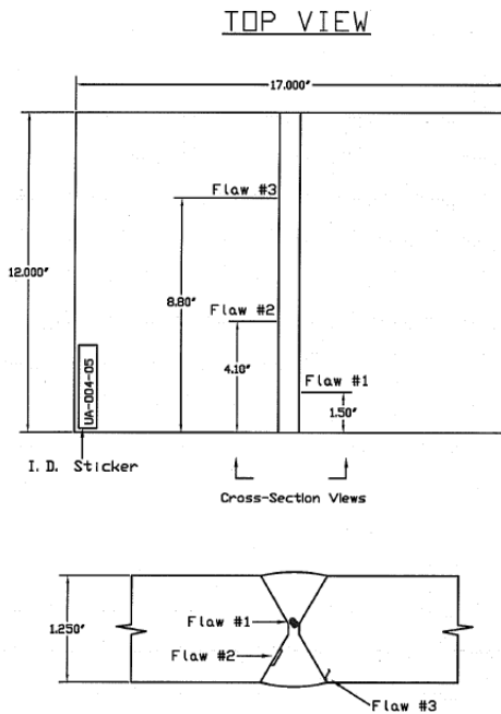
Figure A-2: Details depicting the SMB 11 plate defect locations
