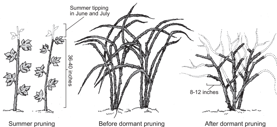
Figure 3. Prune summer-fruiting black raspberries, purple raspberries and erect-growing blackberries by removing primocane tips in the summer and thinning in the winter.
