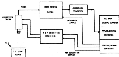
Image Dissector Scanner System (IDS)
