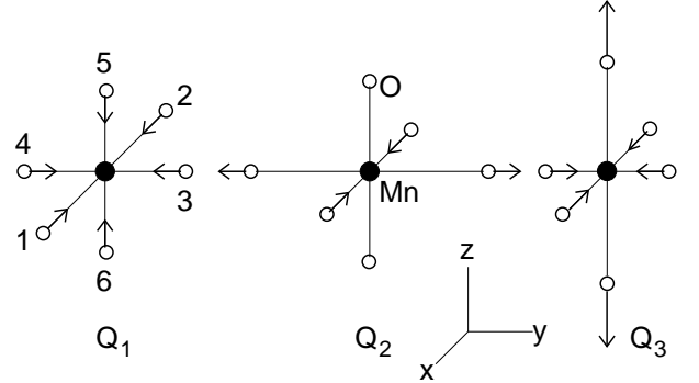
FIG. 3: Vibronic modes for the \text{MnO}_6 octahedron with the eigenvectors: |Q_1\rangle = (-X_1 + X_2 - Y_3 + Y_4 - Z_5 + Z_6)/\sqrt{6} , |Q_2\rangle = (-X_1 + X_2 + Y_3 - Y_4)/2 , and |Q_3\rangle = (-X_1 + X_2 - Y_3 + Y_4 + 2Z_5 - 2Z_6)/\sqrt{12} , where X_1 denotes the x coordinate of the first oxygen atom, etc.
