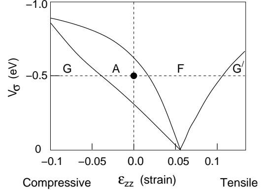
FIG. 1: The ground-state magnetic phase diagram for LMO as a function of strain and the d\delta\sigma electronic hopping V_\sigma , as obtained from our model. Type A represents the phase with ferromagnetic ab planes stacked antiferromagnetically along the c axis, while F and G stand, respectively, for the ferromagnetic and the Néel ordered antiferromagnetic state. We distinguish between two type G states (G and G') depending on the orbital occupancy of the Mn e_g electron: x^2 - 1 or y^2 - 1 for G and z^2 - 1 for G'. For LMO, V_\sigma is about -0.5 eV.
