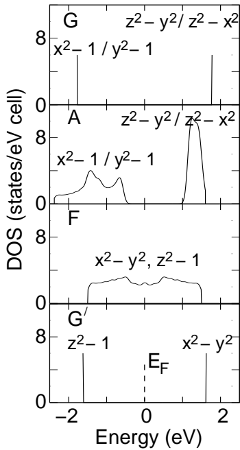
FIG. 8: Densities of states (DOS) corresponding to the four strain conditions of Fig. 2, with hopping parameter V_\sigma = -0.5 eV. In the Néel ordered G and G' phases, complete suppression of hopping leads to the \delta -functions in the DOS; In the G phase, alternate Mn sites have the x^2 - 1 or the y^2 - 1 orbitals occupied with the remaining component of the e_g manifold empty, leading to the checkerboard orbital ordering, while in the G' phase, all sites have the z^2 - 1 orbital occupied. In the A phase, allowed hopping in the plane leads to a broadening of the band, but still a gap in the DOS remains. In the ferromagnetic F phase, hopping both in and out of the plane is strong enough to close the gap, leading to a metallic state due to band gap closure. The Fermi energy is taken as the zero of energy in this plot.
