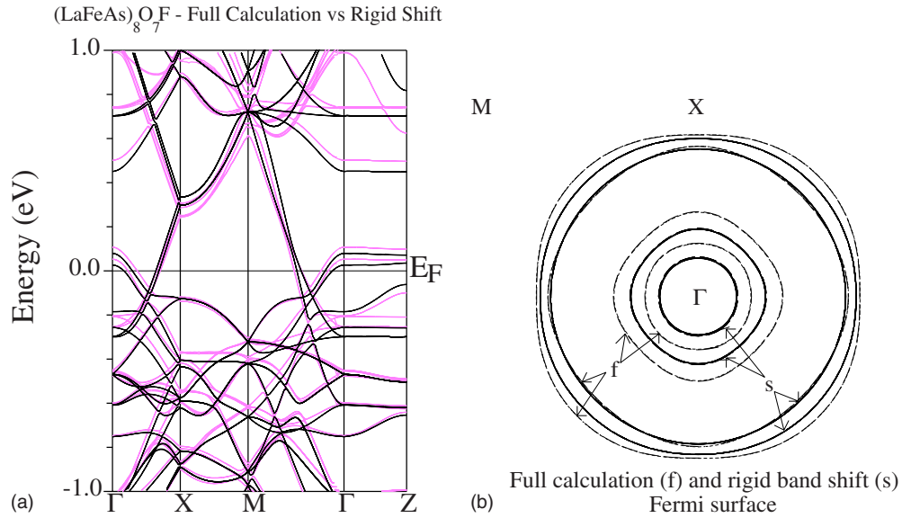
FIG. 3. (Color online) (a) Band structure for the 32-atom NM \text{LaFeAsO} unit cell shown for one F atom replacing O ( \text{La}_8\text{Fe}_8\text{As}_8\text{O}_7\text{F} ) in gray (violet) and for the undoped material ( \text{La}_8\text{Fe}_8\text{As}_8\text{O}_8 ) with rigid shift in black and (b) the corresponding Fermi surfaces given on the \Gamma - X - M plane. The symmetry points are for the supercell Brillouin zone, which has the same symmetry points as in the original unit cell but with half the magnitudes for the k_x and k_y components.
