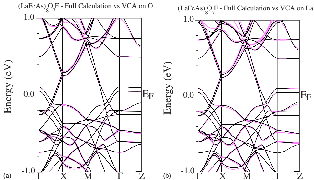
FIG. 4. (Color online) (a) Supercell band structure of fluorine-doped \text{LaFeAsO} ( \text{La}_8\text{Fe}_8\text{As}_8\text{O}_7\text{F} ) [gray (violet) lines] compared with the equivalent VCA calculation (black lines) with changed O nuclear charge. (b) Same as (a) except that the VCA calculation was done with changed La nuclear charge (black lines). No difference is seen between the two sets of band structures near E_F .
