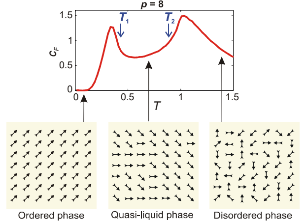
FIG. 2 (color online). Three-phase regime for p = 8 , in terms of the specific heat, c_F , transition temperatures T_1, T_2 (the transitions do not occur at the peaks of c_F ), and typical spin configurations. The correlation function, \langle \mathbf{s}_i \cdot \mathbf{s}_j \rangle , goes to a non-zero constant at large distance |i - j| , at T < T_1 (long-range order), decays as a power law of distance at T_1 < T < T_2 (quasi-long-range order [5,6]; typical configurations contain vortices, such as the clockwise vortex fragment in the center panel), and decays exponentially with distance at T > T_2 (disorder).
