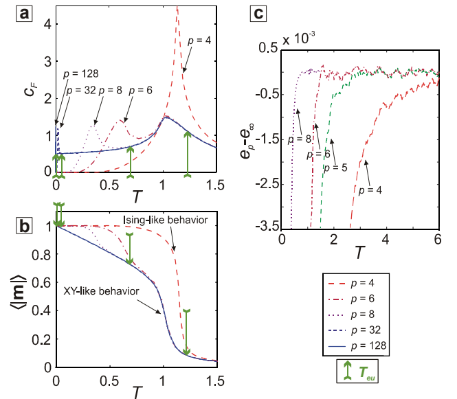
FIG. 3 (color online). Heat capacity (a), magnetization (b), and difference of internal energy per spin relative to the planar rotor model (c). The data correspond to a system size of L = 72 ( N = 5,184 spins). All curves coalesce above T_{eu} (arrows) for p \geq 5 (collapse of thermodynamic observables, extended universality).
