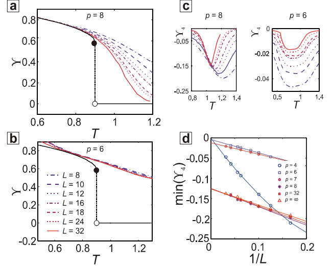
FIG. 4 (color online). Helicity modulus, \Upsilon , and fourth-order helicity, \Upsilon_4 , for p=8 (a, c) and p=6 (b, c) across the phase transition T_2 . The bottom curve in (a, b), for reference, is the modulus for the planar rotor, which jumps from 2T_{\text{BKT}}/\pi (full circle) to zero at T = T_{\text{BKT}} . For all p \geq 8 , \lim_{L \rightarrow \infty} \Upsilon = 0 . Extrapolation of \Upsilon_4 to the thermodynamic limit yields two classes of results (d): \Upsilon_4 converges to the universal value -0.126 \pm 0.005 for p \geq 8 , and to zero for p \leq 7 . This implies that \Upsilon has a discontinuous jump to zero at T_2 if and only if p \geq 8 (see text).
