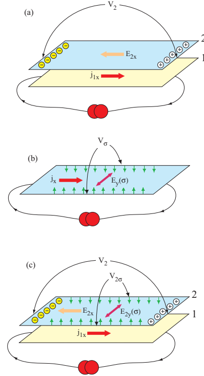
FIG. 1: (Color online) (a) In ordinary Coulomb drag the current j_{1x} in layer 1 induces, via inter-layer Coulomb interaction, an electrochemical potential gradient E_{2x} in layer 2. (b) In spin Hall effect the current j_x in a single layer induces, via spin-orbit interaction, a spin-dependent electrochemical potential gradient E_y(\uparrow) = -E_y(\downarrow) causing electrons of opposite spin orientation to accumulate on opposite edges. (c) In Spin Hall drag the current j_{1x} in layer 1 induces, via a combination of inter-layer Coulomb interaction and spin-orbit interaction, electrochemical potential gradients E_{2x} along layer 2, and E_{2y}(\sigma) across layer 2.
