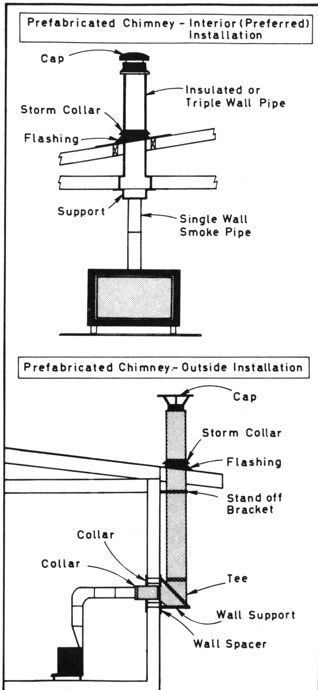
Figure 3. Two alternative methods of installing prefabricated chimneys.
