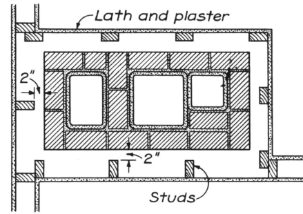
Figure 4. Chimney with proper arrangement of three flues. Bond division wall with sidewalls by staggering the joints of successive courses. Wood framing should be at least 2 inches from brickwork.
