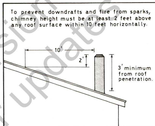
Figure 1. Required roof clearances.
