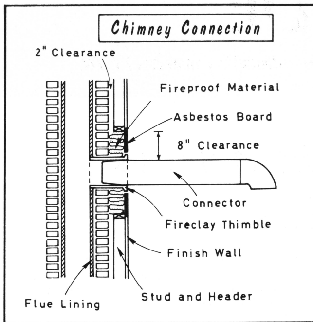
Figure 2. Proper method of connecting stove pipe to the chimney.
