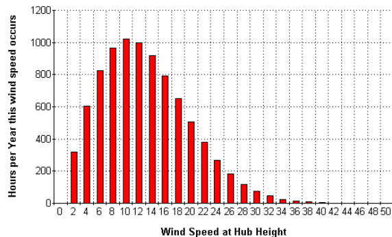
WIND SPEED DISTRIBUTION typical for 13 mph average
