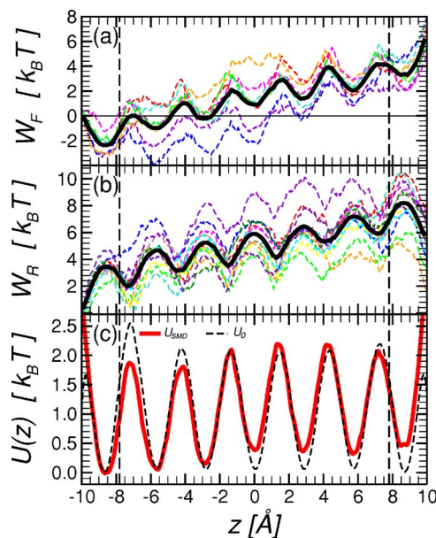
FIG. 4. (Color online) Work along (a) forward and (b) reverse SMD pullings (dashed lines). The mean work \bar{W}_{F/R} is shown as thick-solid line. (c) Comparison between U_0(z) (dashed line) and U_{FR}(z) = (\bar{W}_F - \bar{W}_R)/2 (solid line), obtained from fast forward and reverse SMD pullings. Vertical dashed lines indicate the extremities of SWNTs.
