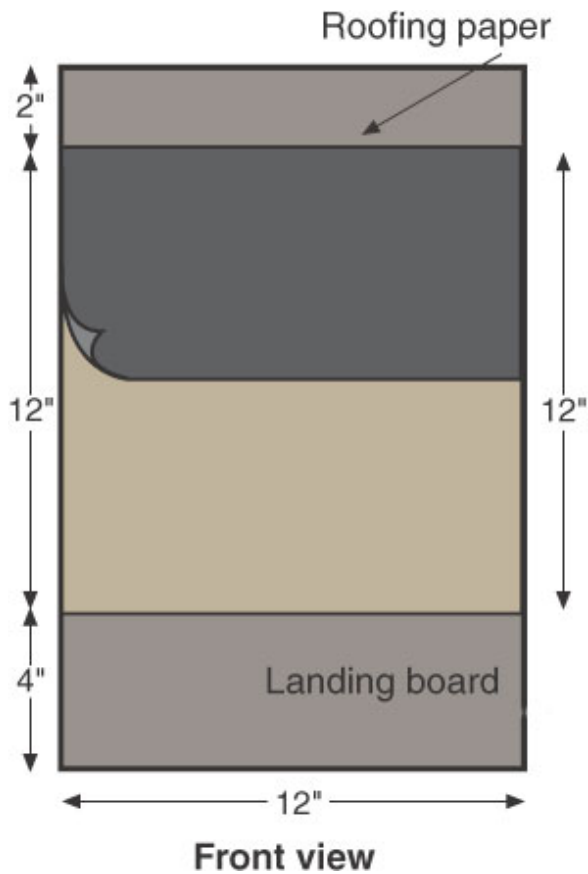
Figure 5 Beginner's bat house.
