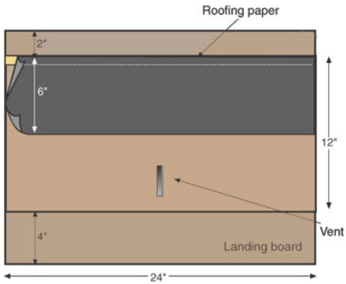
Figure 6 A small nursery bat house.
