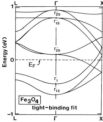
FIG. 7. Nearest-neighbor tight-binding fit to the LMTO minority bands near Fermi energy. The LMTO bands are shown in Fig. 6.
