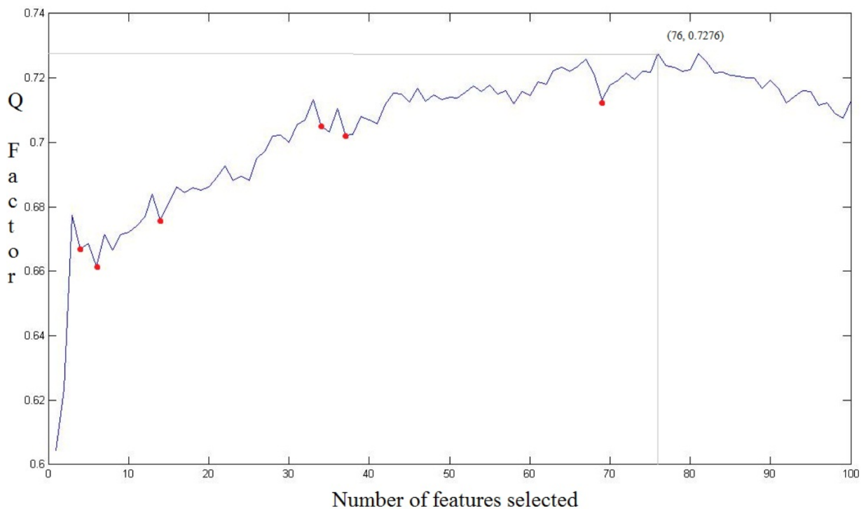
Figure 8: Quality factor verses number of features using a best-first wrapper with naïve Bayesian OVR. Q peaks at 0.728 using the first 76 features from ROC-AUC ranked WPC.
