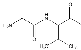
Glycine-Valine
